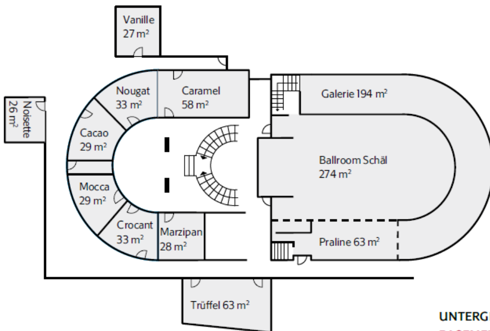
ERDGESCHOSS GROUND FLOOR
