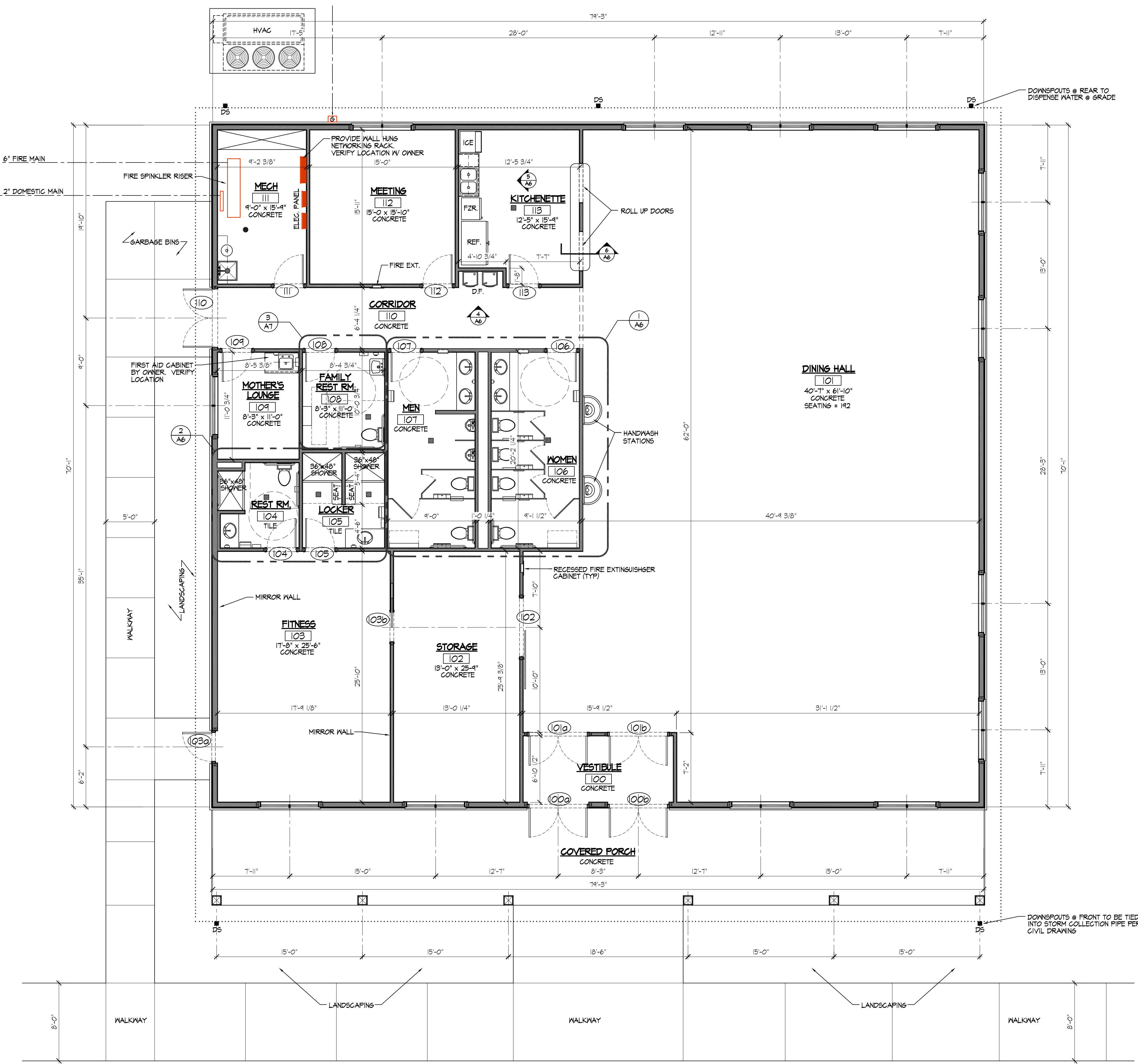
FLOOR PLAN SQUARE FEET = 5,585
